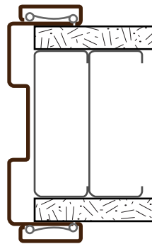
Jamb - Inverted Stop
