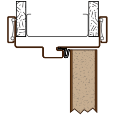
3D Header - Kerfed
